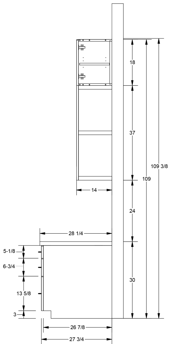
Cross Section through center cabinets and suspended shelves
