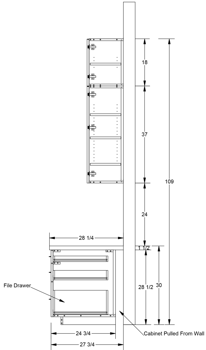
Cross Section through base cabinet and both wall cabinets
